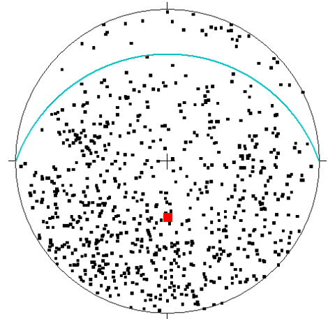
Stereographic plot of 762 randomly oriented microfaults measured in drillcore from holes plunging 60°S (red square).
